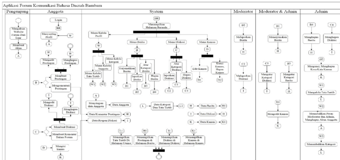
Gambar 2 Activity diagram
